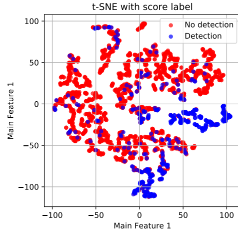
(d) Clustering using t-SNE to reduce dimensionality and score threshold to label.
