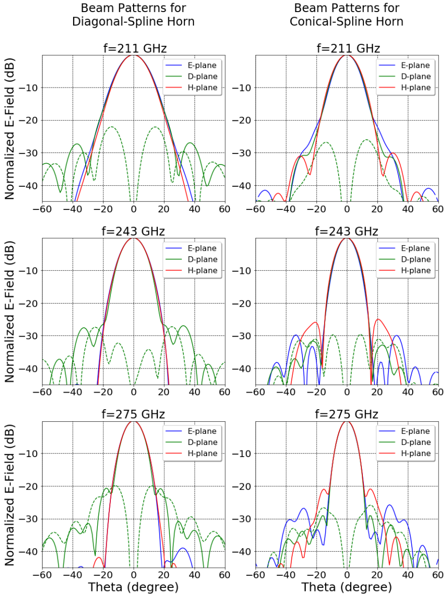
FIGURE 4.3: Simulated radiation beam pattern
