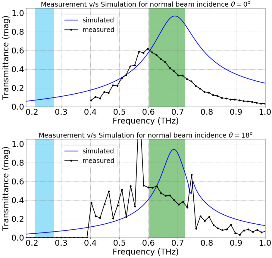
FIGURE 3.18: Experimental results for JC dichroic
