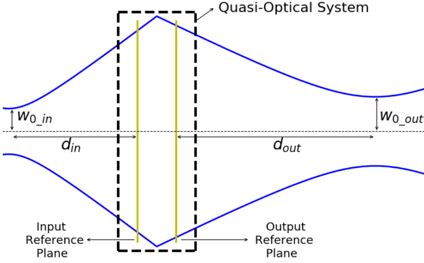
FIGURE 2.7: Transformation of a Gaussian-beam.
