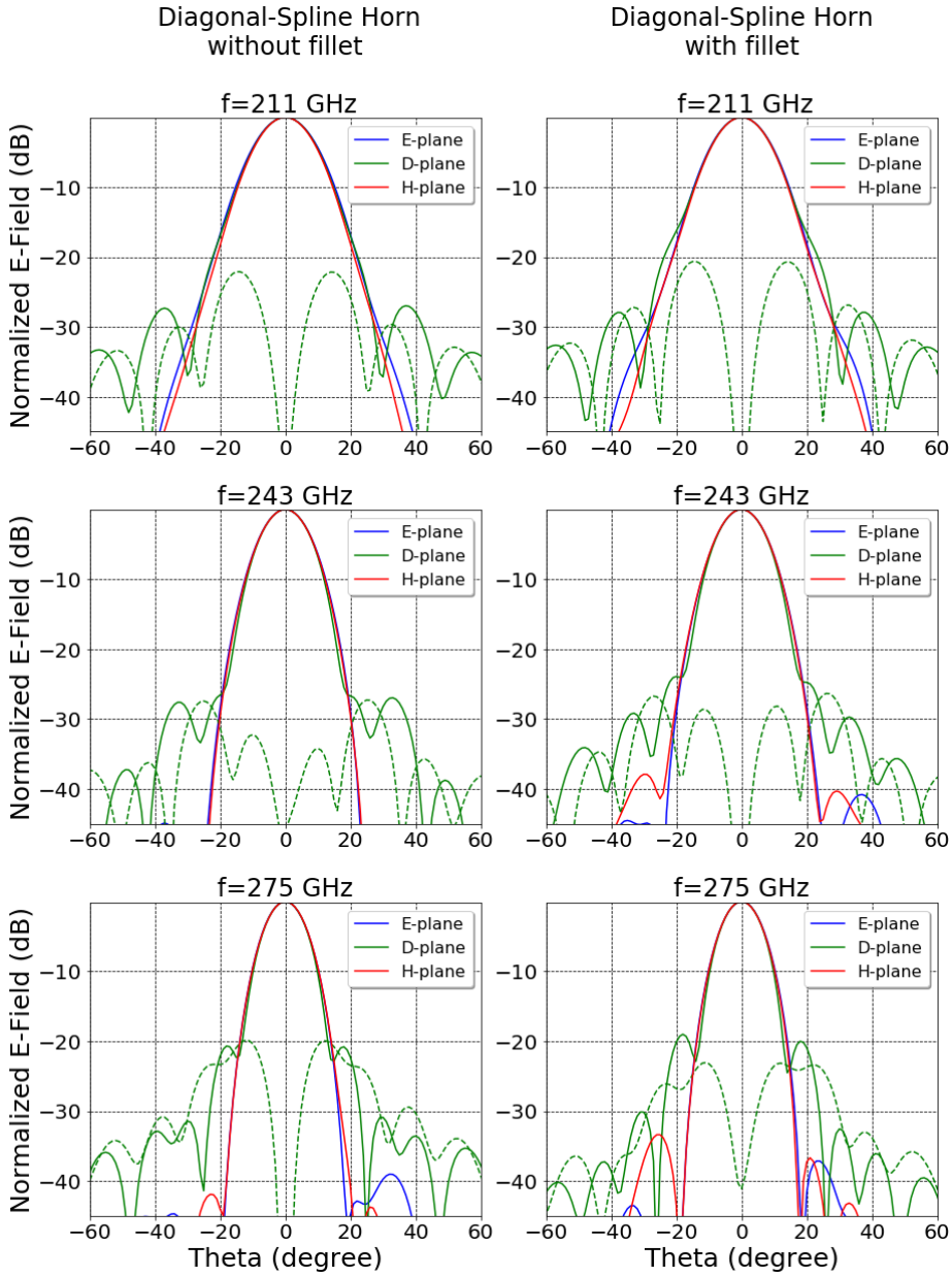
FIGURE 4.7: Simulated far field radiation pattern
