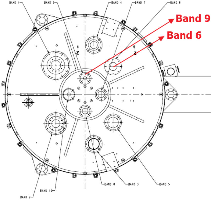
FIGURE 2.1: ALMA cryostat layout
