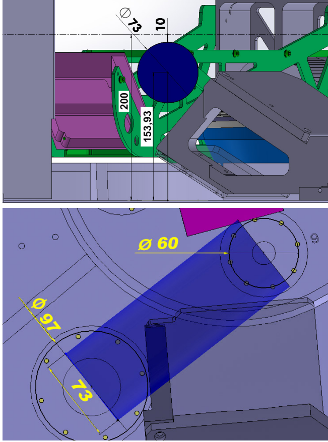
FIGURE 2.5: The Safe Work Zone
