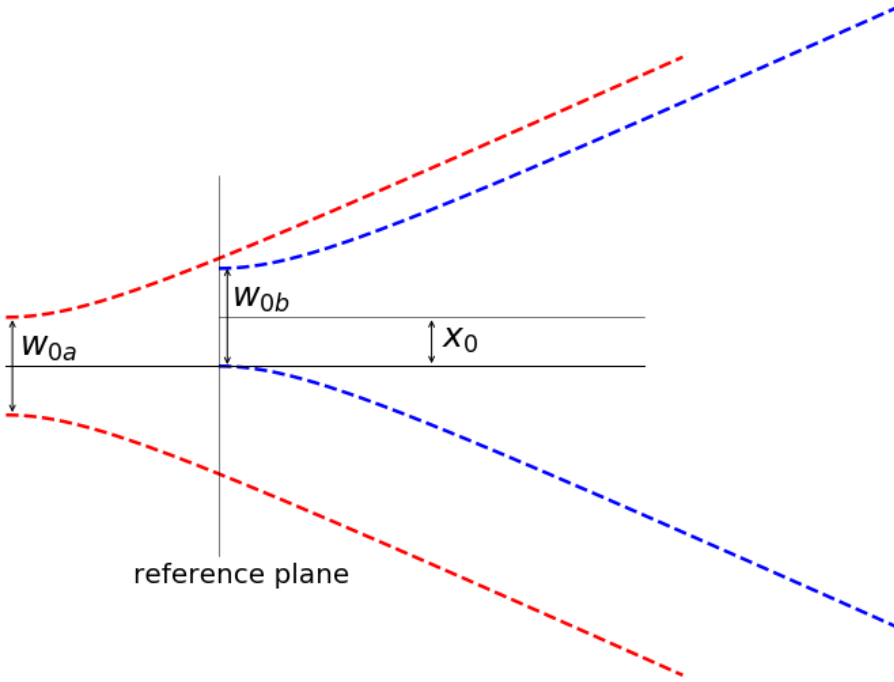
FIGURE 2.11: Offset beam mismatch
