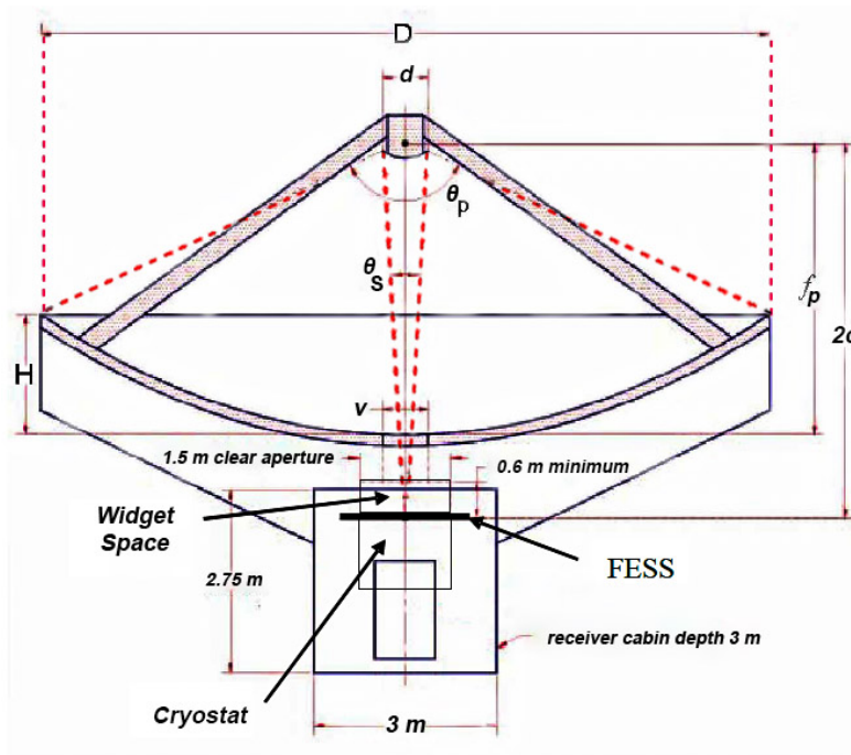
FIGURE 1.8: Schematic of an ALMA antenna.
