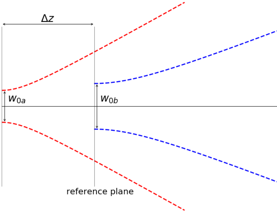
FIGURE 2.9: Axially aligned beam mismatch
