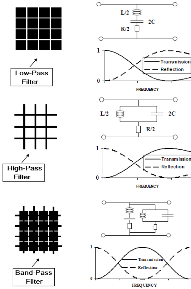
FIGURE 3.3: Metallic grids and their equivalent circuits
