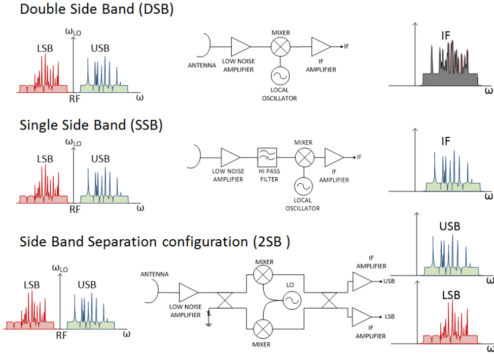
FIGURE 1.3: Types of heterodyne receivers
