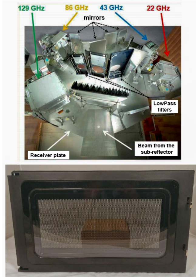
FIGURE 3.2: Applications of dichroic filters
