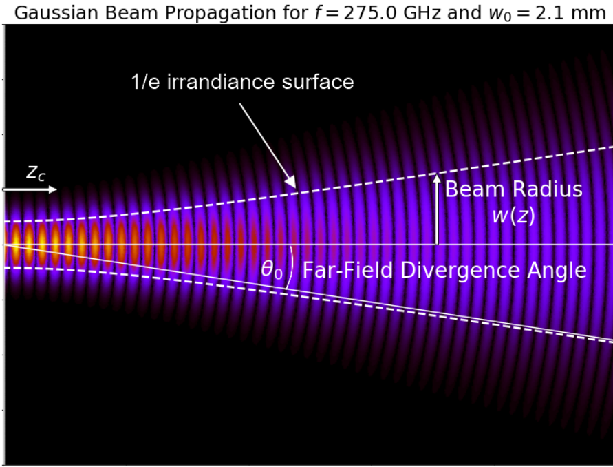
FIGURE 2.6: Gaussian beam representation.
