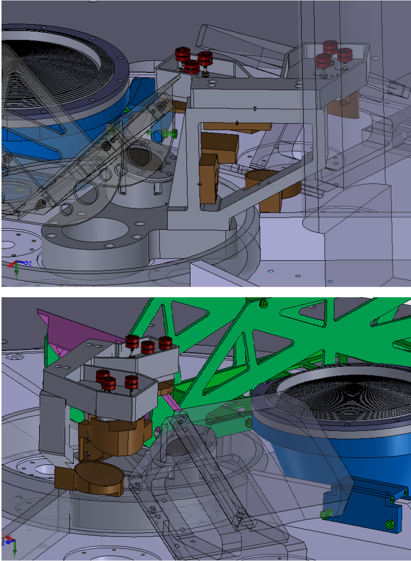
FIGURE 2.19: Rendering of the beam combiner system once is mounted on the cryostat
