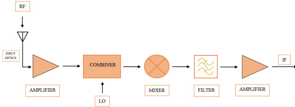
FIGURE 1.2: Types of heterodyne receivers
