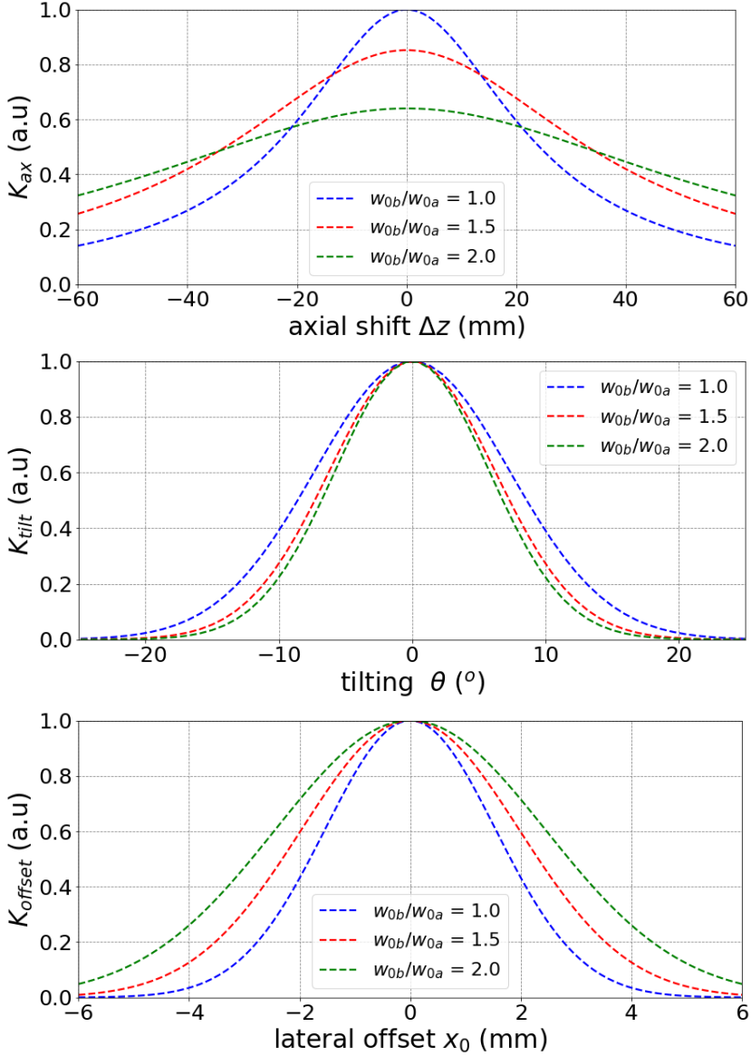
FIGURE 2.16: Coupling Efficiency Analysis
