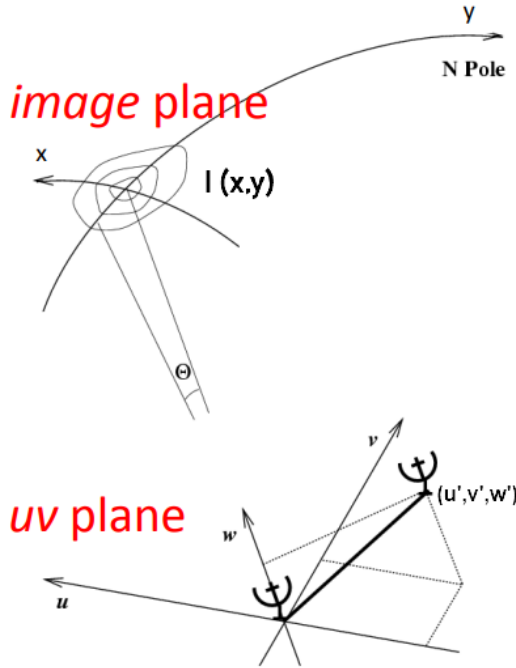
FIGURE 1.5: Relationship between uv-plane and image plane.
