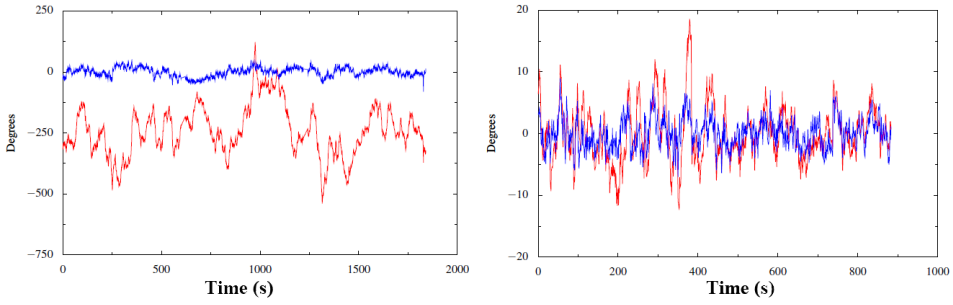
FIGURE 1.14: Atmospheric calibration problem.
