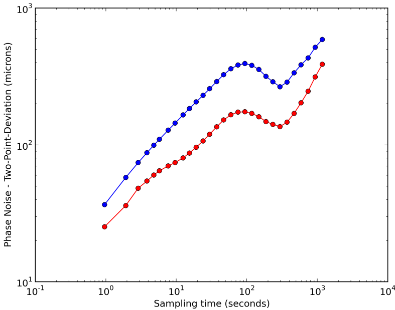
FIGURE 1.11: Temporal dependence of atmospheric fluctuation
