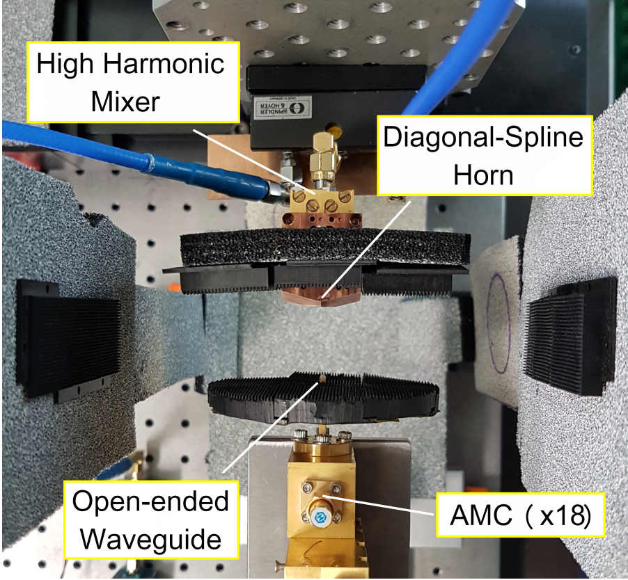
FIGURE 4.13: Experimental set-up to measure near-field radiation pattern
