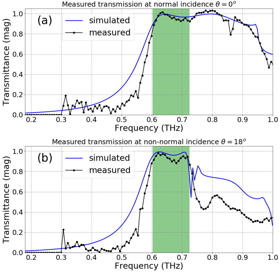
FIGURE 3.15: Experimental results for FT dichroic
