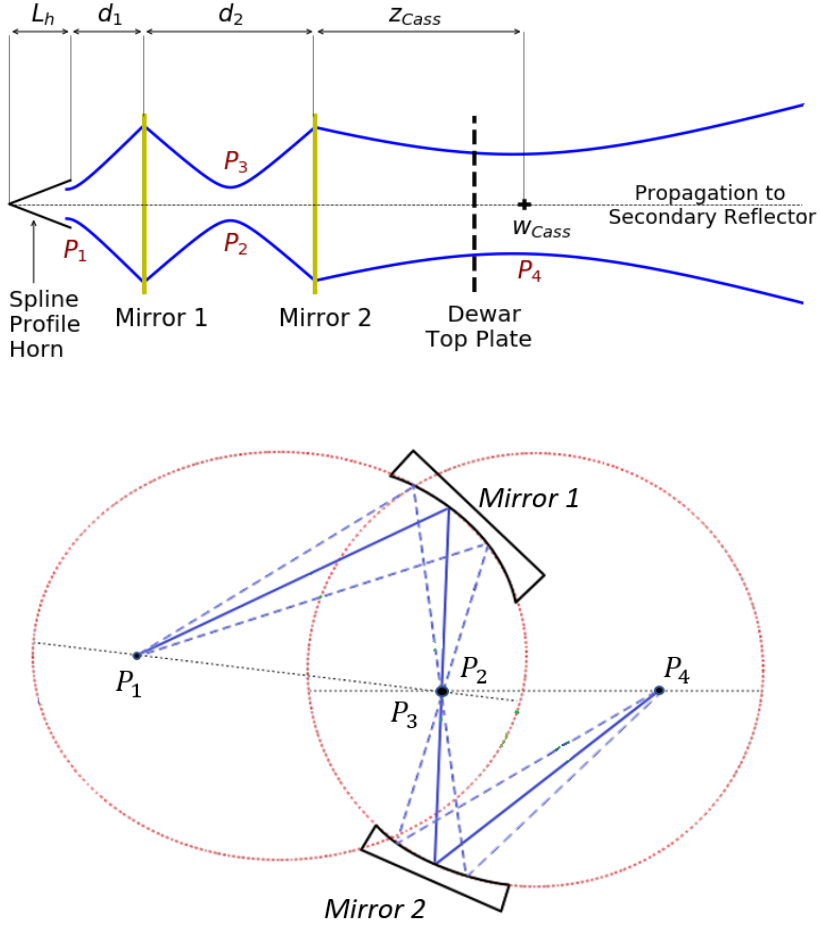
FIGURE 4.5: Optical train description of the ALMA cold optics
