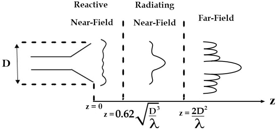
FIGURE 4.11: The propagation regions of an electromagnetic beam
