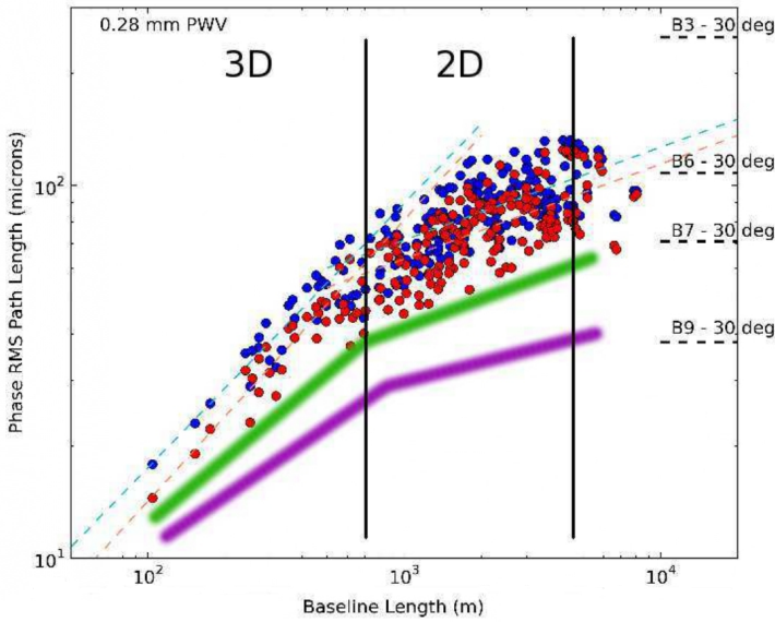
FIGURE 1.12: Spatial dependence of atmospheric fluctuation
