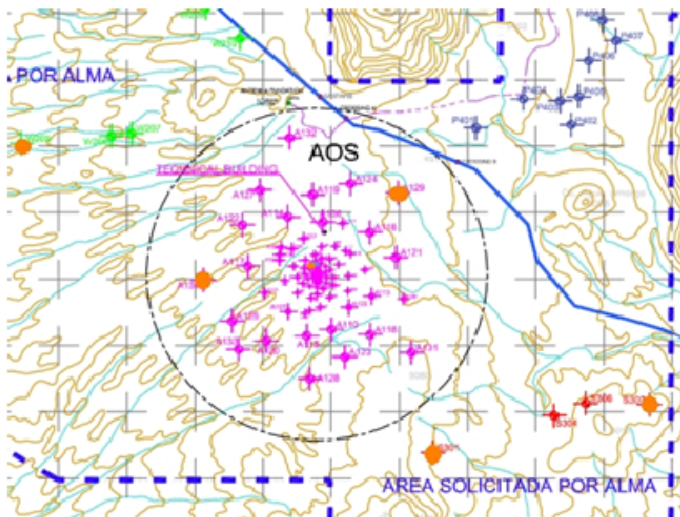
FIGURE 1.13: Antennas paired for sub-array experiment
