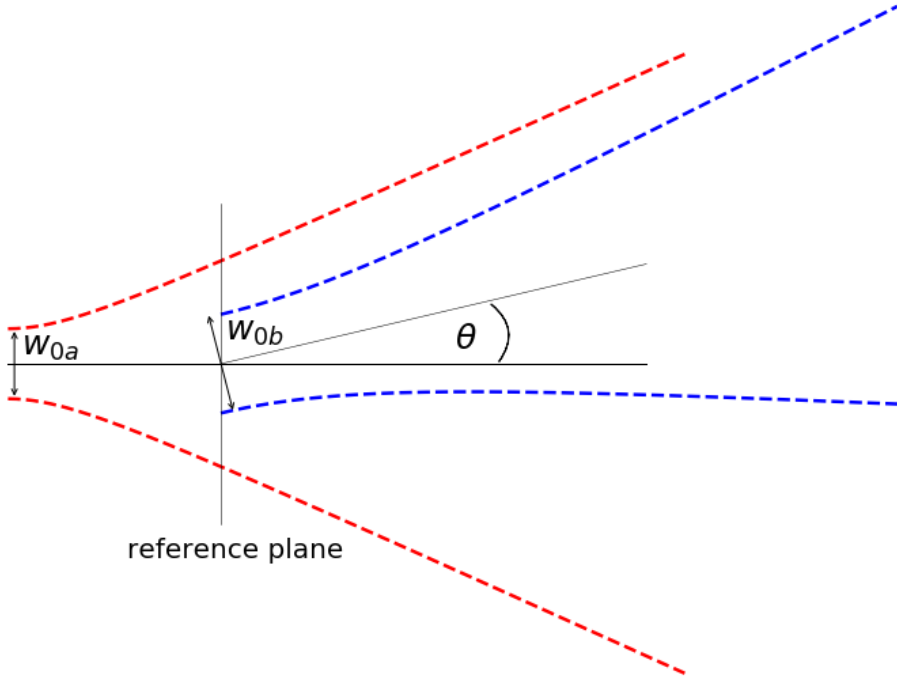
FIGURE 2.10: Tilted beam mismatch
