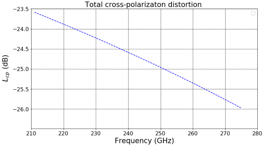
FIGURE 2.13: Cross polarization distortion calculation
