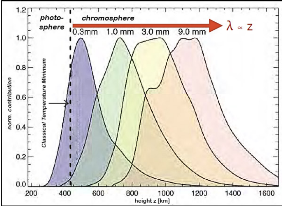
FIGURE 1.15: Contribution functions of the continuum intensity
