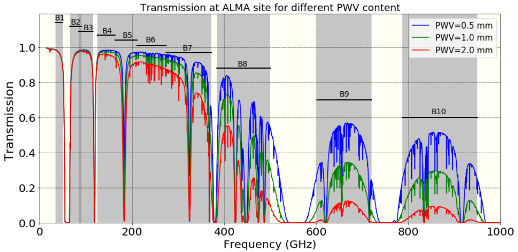
FIGURE 1.1: Atmospheric windows at Chajnantor.
