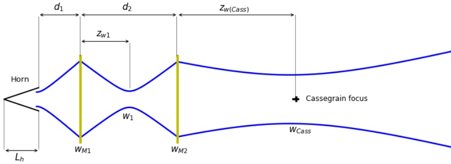
FIGURE 2.2: Optical train representation.
