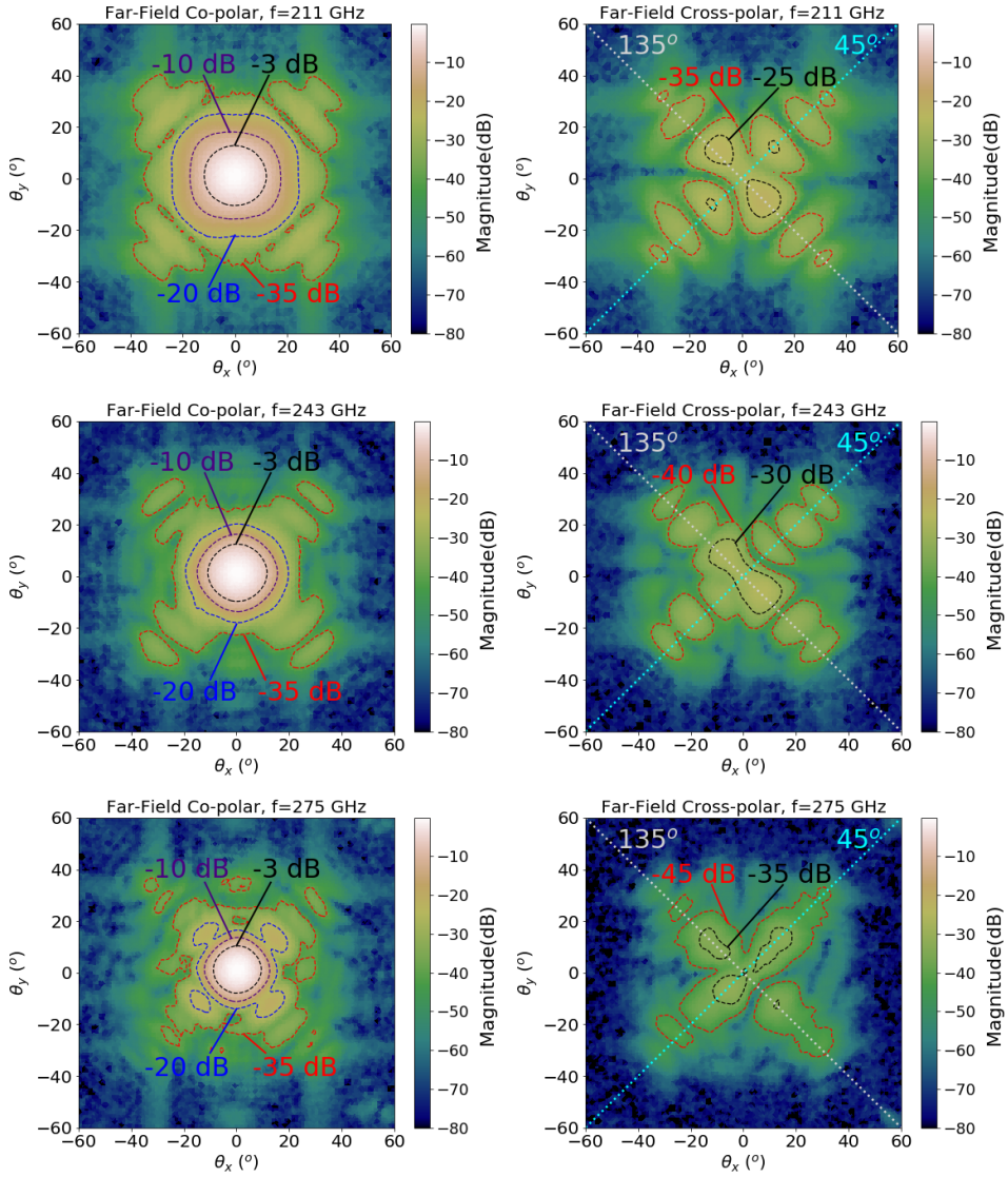
FIGURE 4.14: Experimental results for far field radiation pattern
