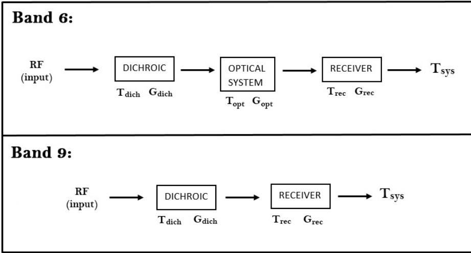
FIGURE 2.14: Resulting cascade system for each receiver,
