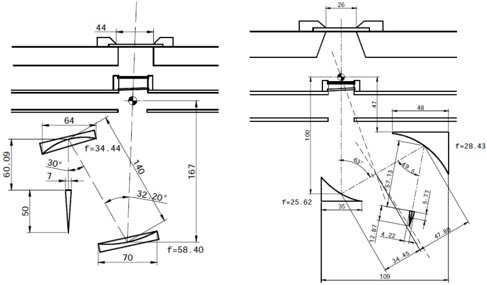
FIGURE 2.3: Cold optics drawing of Band 6 and 9.
