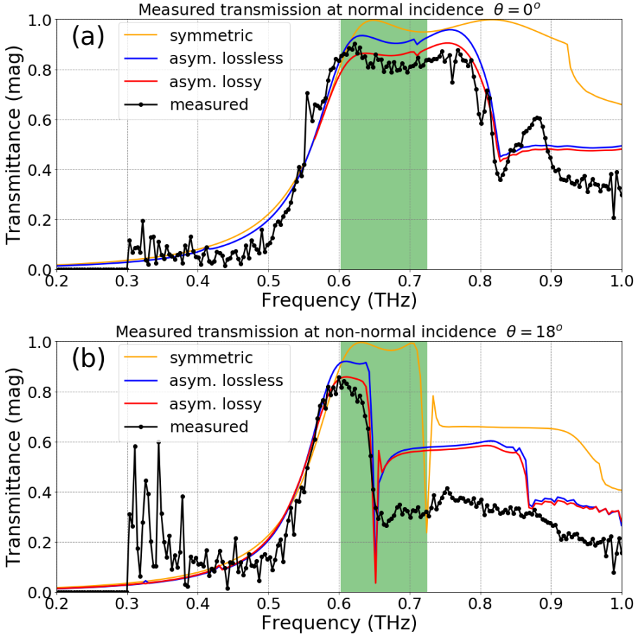
FIGURE 3.16: Experimental results for SH dichroic
