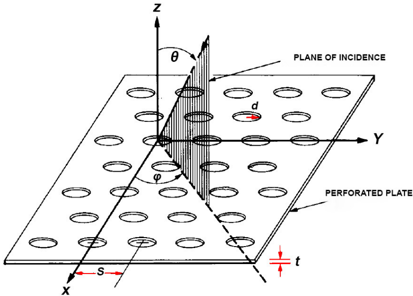
FIGURE 3.1: Dichroic plate geometry
