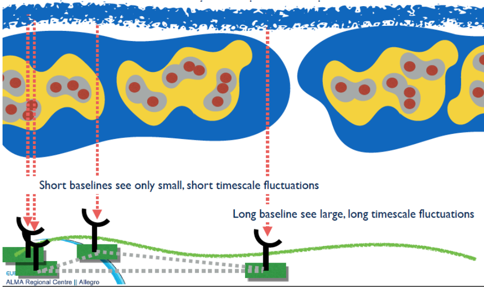
FIGURE 1.9: Atmospheric distortion producing loss of coherence
