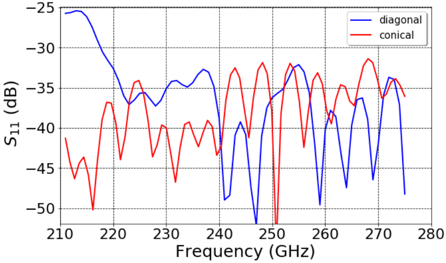
FIGURE 4.4: Simulated return loss
