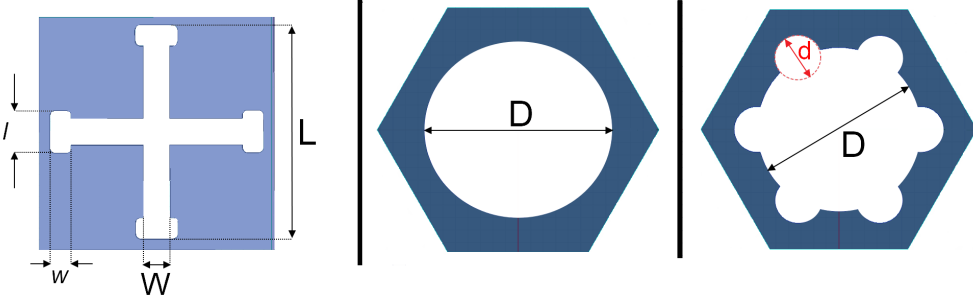
FIGURE 3.5: Proposed configurations for a dichroic filter
