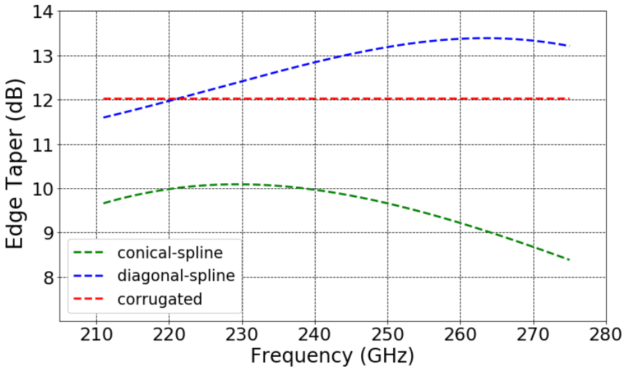
FIGURE 4.6: Edge taper versus frequency
