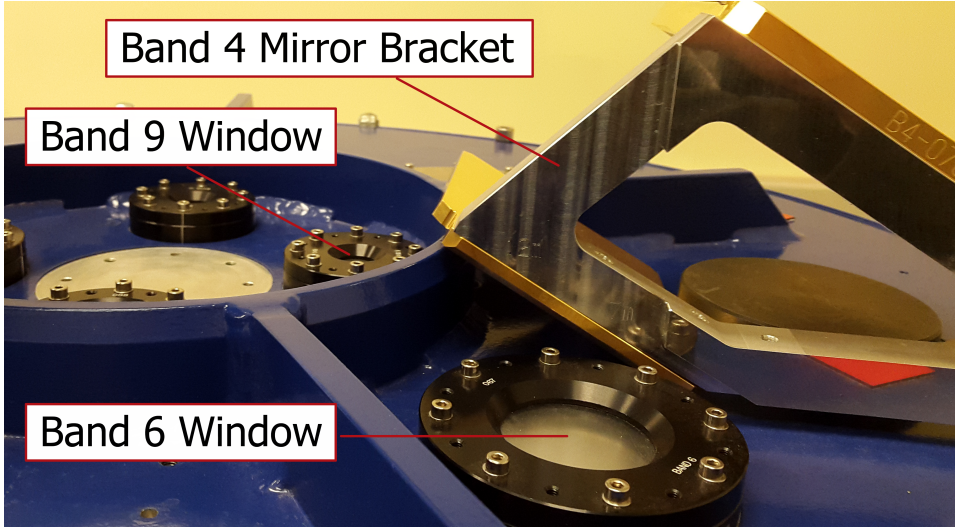
FIGURE 2.4: Images of the cryostat.
