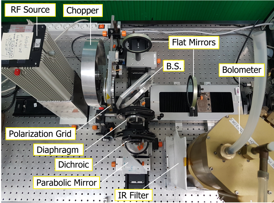
FIGURE 3.14: FTS experimental set-up.
