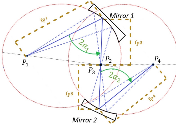
FIGURE 2.8: General elliptical mirror configuration.
