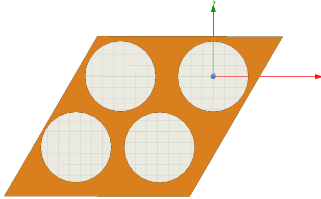
FIGURE 3.17: Implemented super-cell
