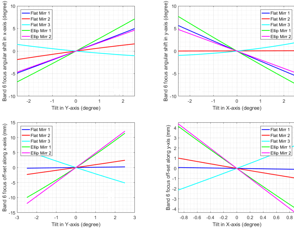
FIGURE 2.17: Tolerance Analysis
