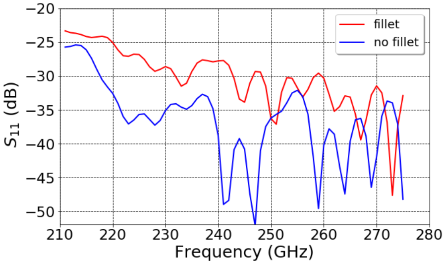
FIGURE 4.8: Return loss comparison.
