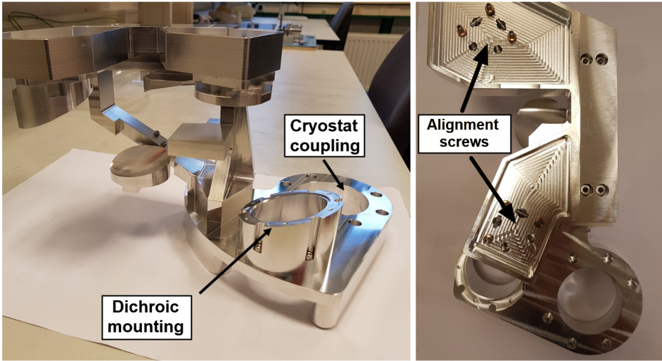
FIGURE 2.20: Constructed beam combiner optical system
