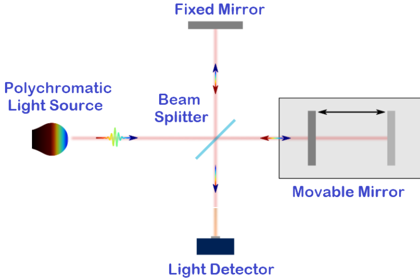
FIGURE 3.12: Michelson Interferometer
