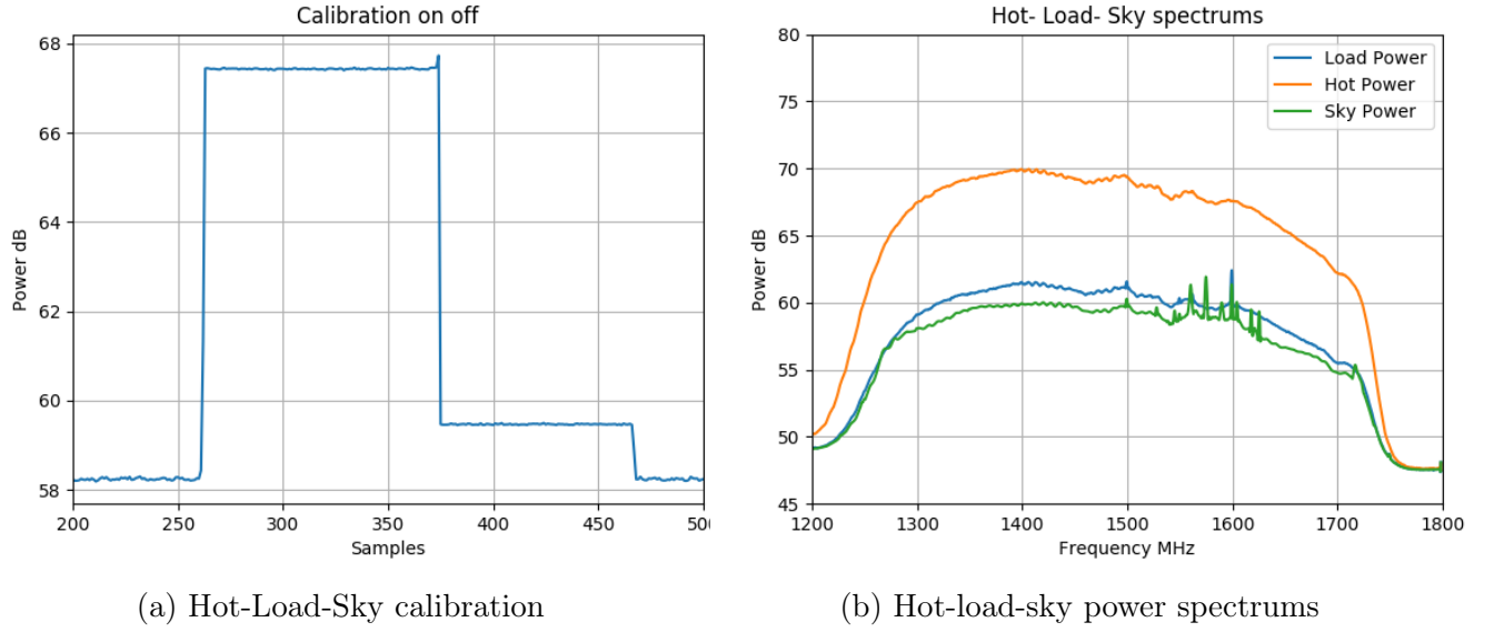
Figure 3.18: Hot-load-sky calibration
