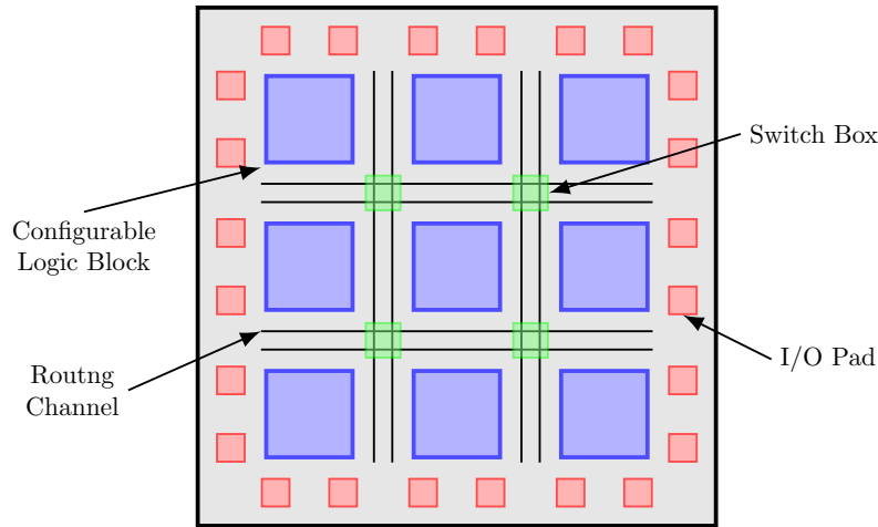
Figure 2.5: FPGA diagram [18]
