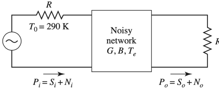
Figure 2.17: Noisy network [27].
