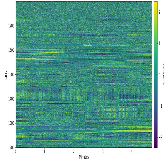
(b) RFI spectrum obtained at Sta Martina
