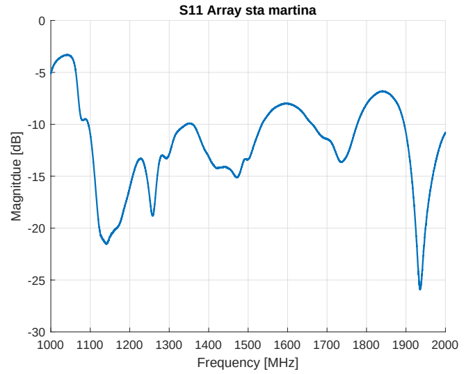
(b) Input reflection coef of an array antenna used.
