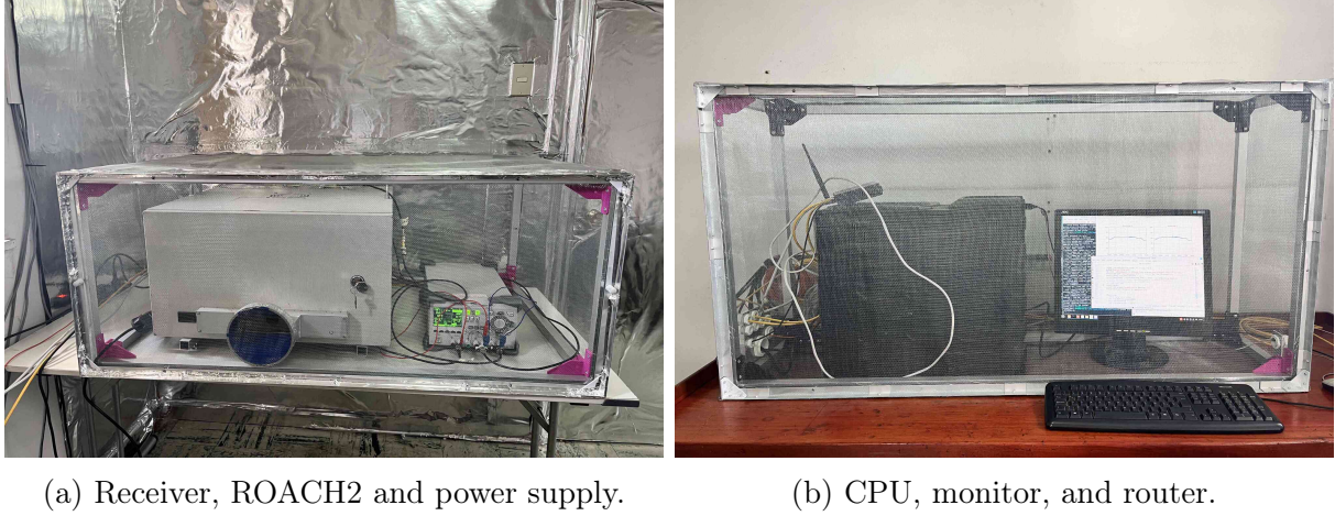
Figure 4.2: Two Faraday cages built to isolate the above equipment.
