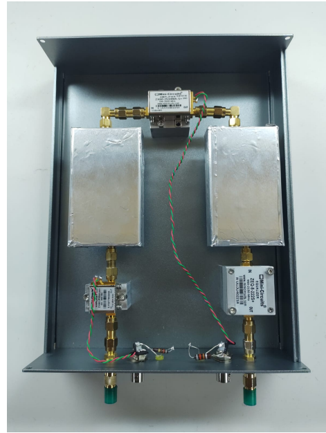
(b) Top view microwave receiver
