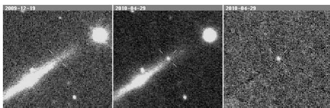
Supernova 2010cl
