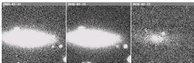
Supernova 2010ac
