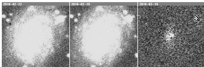
Supernova 2010as
