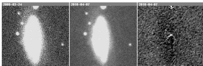
Supernova 2010bk
