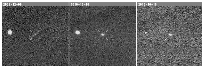
Supernova 2010iv
