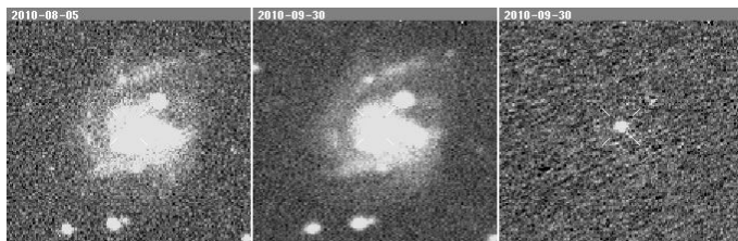
Supernova 2010il
