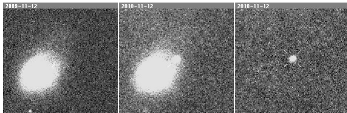
Supernova 2010jr
