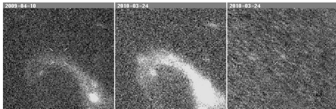
Supernova 2010bi
