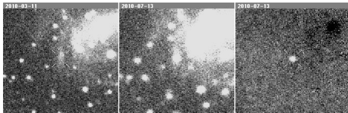
Supernova 2010gh
