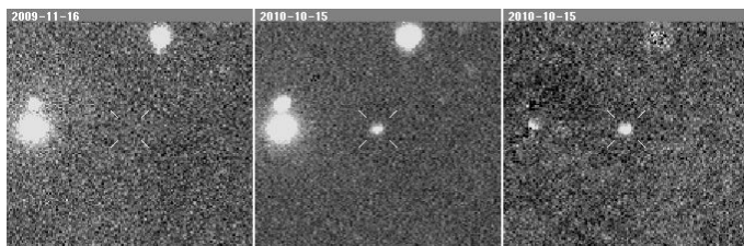
Supernova 2010iu
