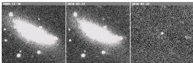
Supernova 2010ae
