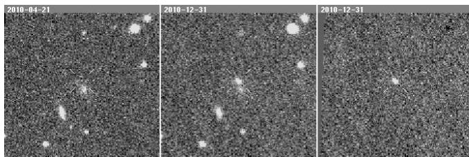
Supernova 2010lv
