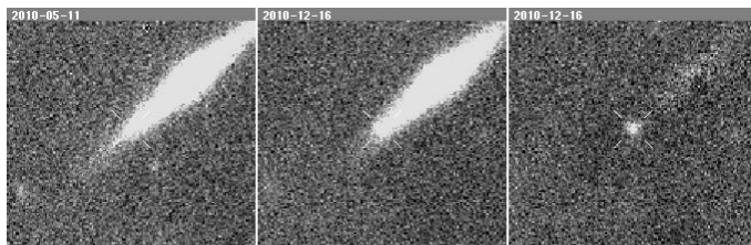
Supernova 2010ku
