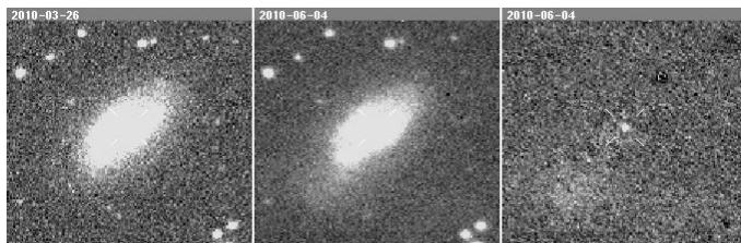
Supernova 2010ds
