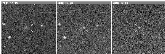
Supernova 2010lm
