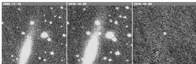
Supernova 2010ir
