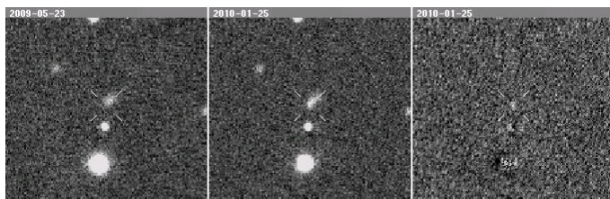
Supernova 2010T
