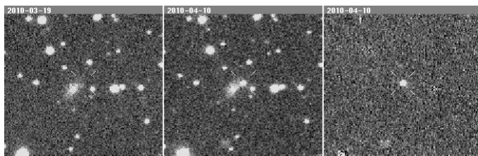
Supernova 2010bo
