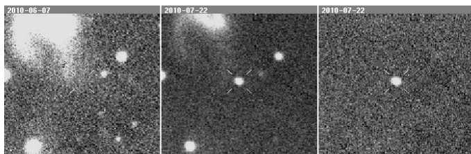
Supernova 2010gp
