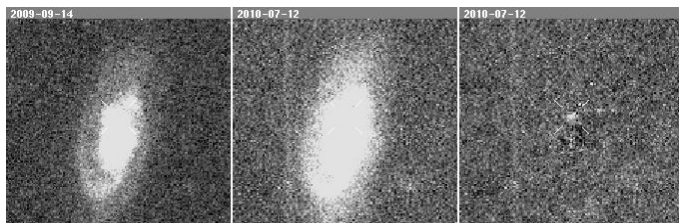
Supernova 2010gg
