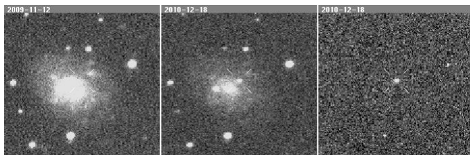
Supernova 2010kw
