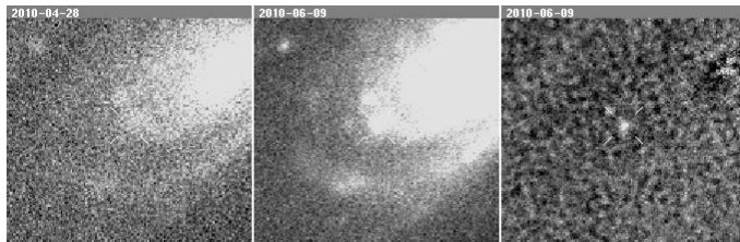
Supernova 2010dx
