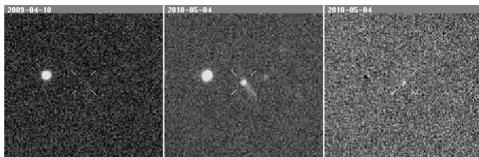
Supernova 2010cn
