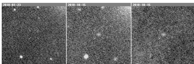
Supernova 2010ja
