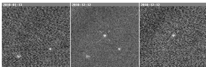
Supernova 2010kt
