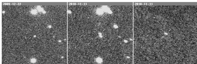
Supernova 2010jp
