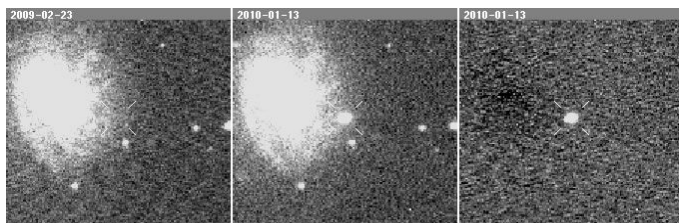
Supernova 2010F
