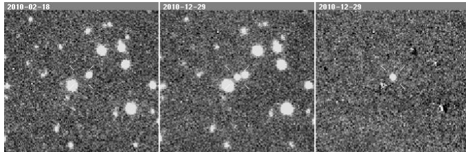
Supernova 2010ls
