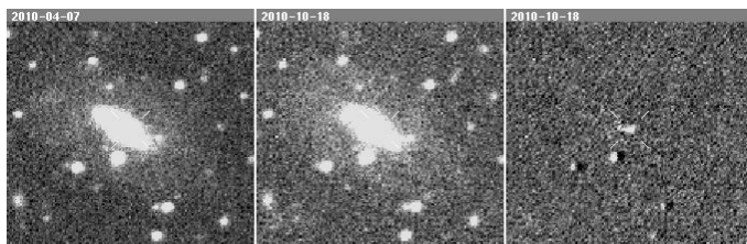
Supernova 2010iy
