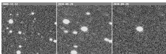
Supernova 2010ih
