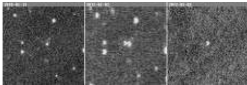
Supernova 2012bc
