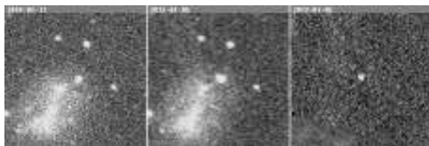
Supernova 2012R
