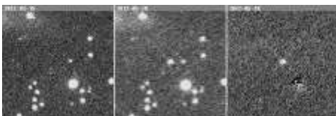
Supernova 2012d
