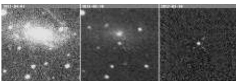
Supernova 2012bt
