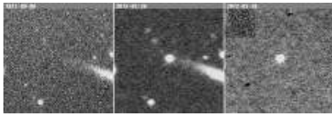
Supernova 2012bl
