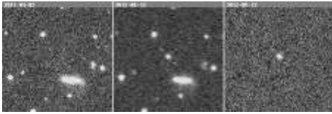
Supernova 2012fy
