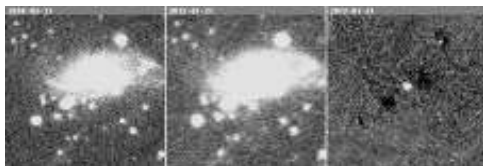
Supernova 2012ba
