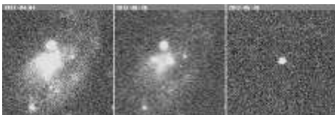
Supernova 2012dh
