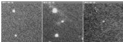
Supernova 2012bk
