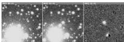
Supernova 2012hs
