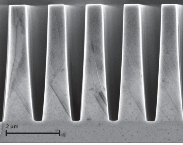
Fig. 4. SEM picture of the cleaved subwavelength grating, from which are deduced the geometric parameters of the AGPM-L4 profile: line width \approx 0.58 \mu\text{m} (i.e., filling factor \approx 0.41 ) and depth \approx 4.7 \mu\text{m} .
