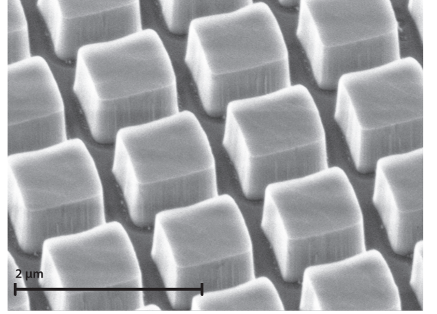
Fig. 5. SEM picture of the antireflective grating (ARG) etched on the backside of the AGPM.
