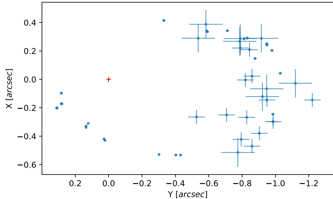
Astrometry
