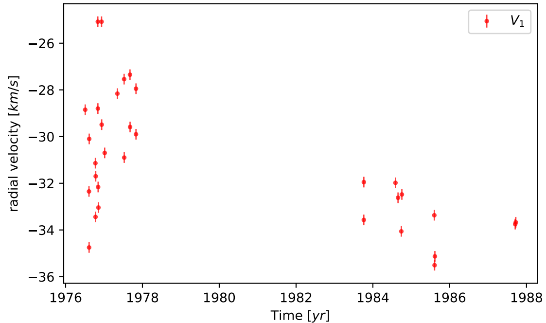
Spectroscopy
