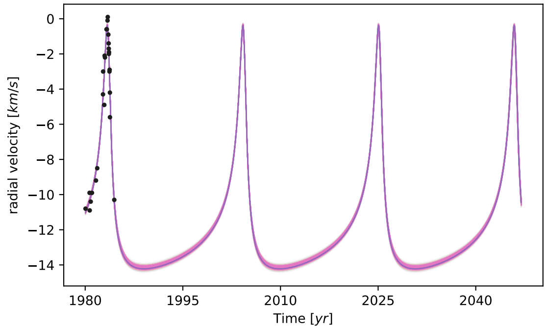
Radial Velocity
