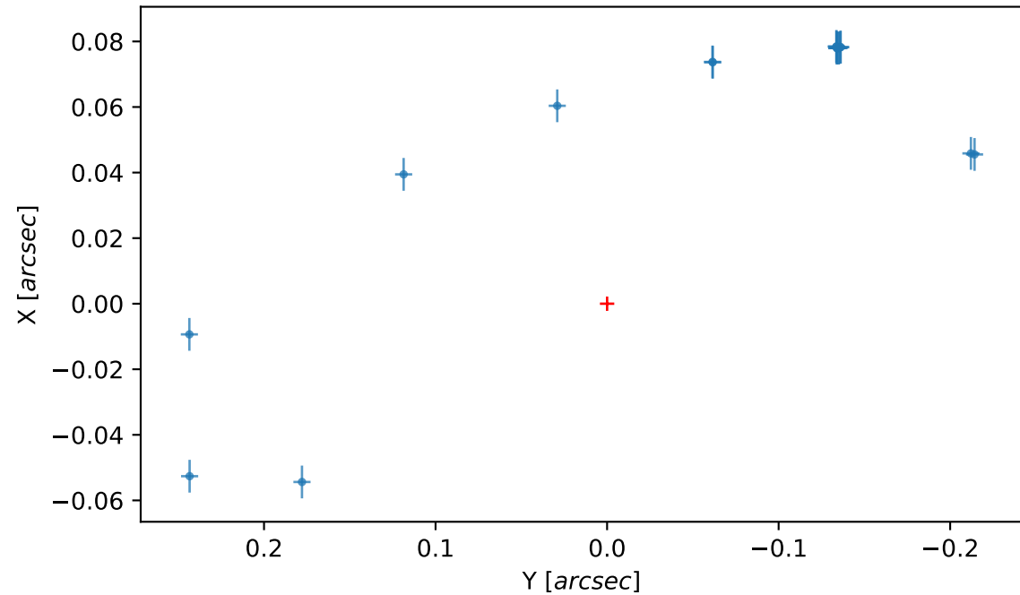
Astrometry
