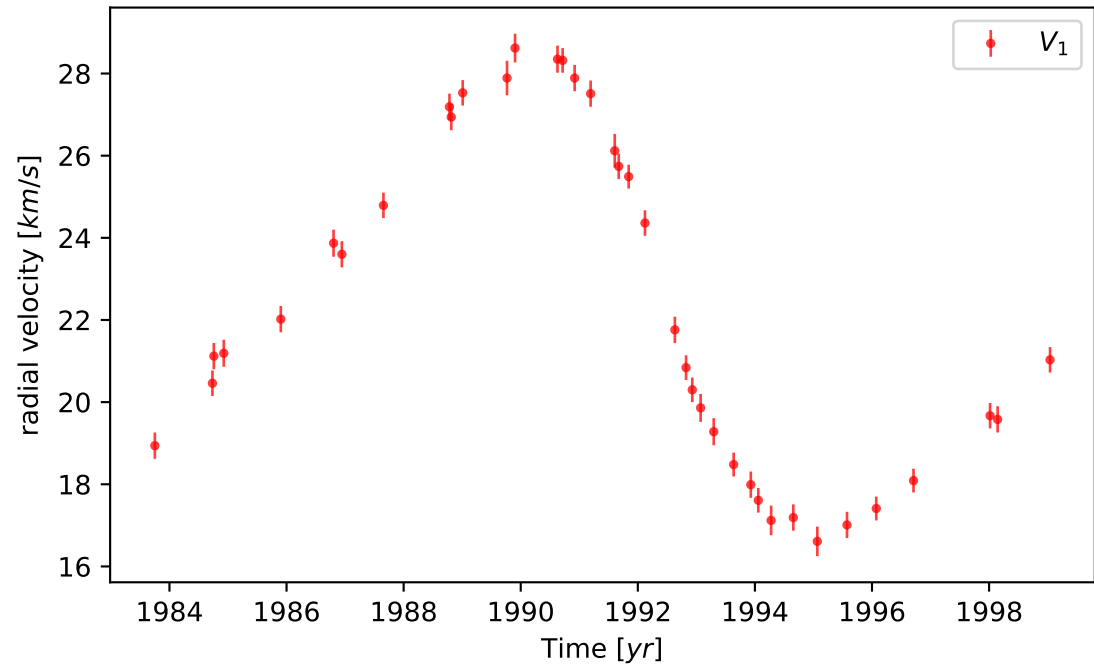
Spectroscopy
