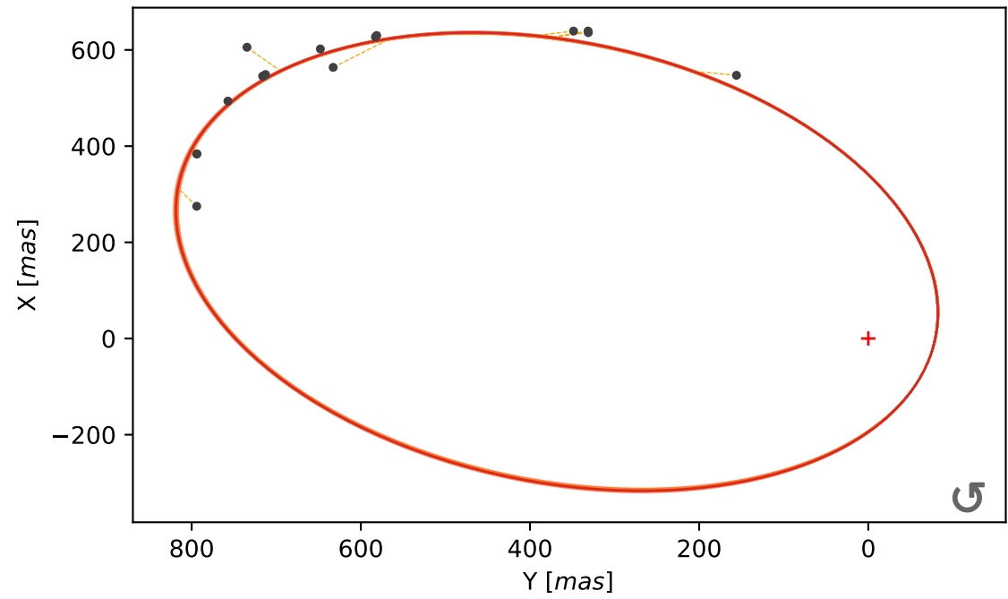
Orbit
