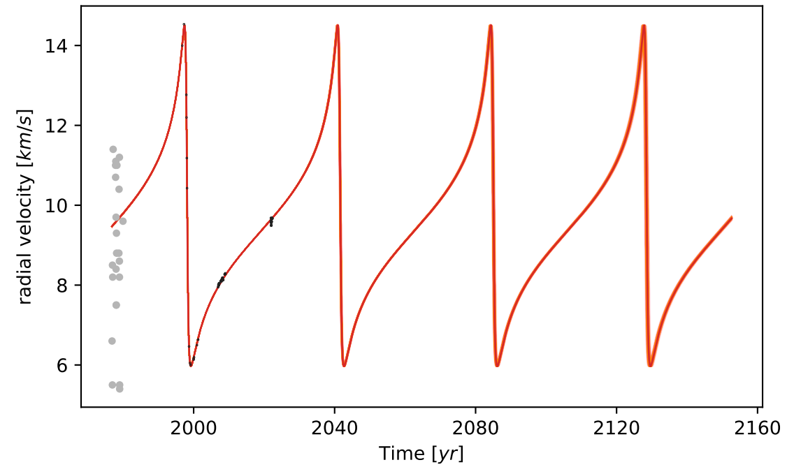
Radial Velocity
