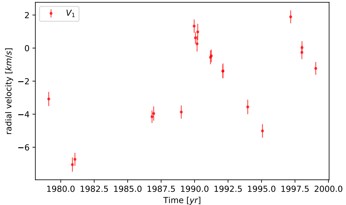
Spectroscopy
