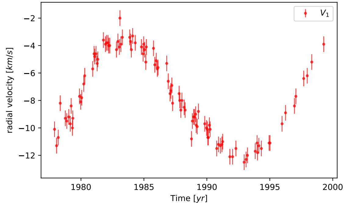
Spectroscopy
