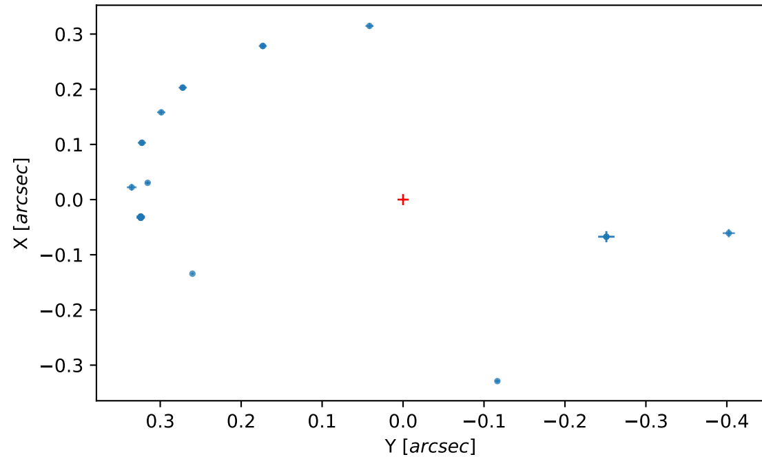
Astrometry
