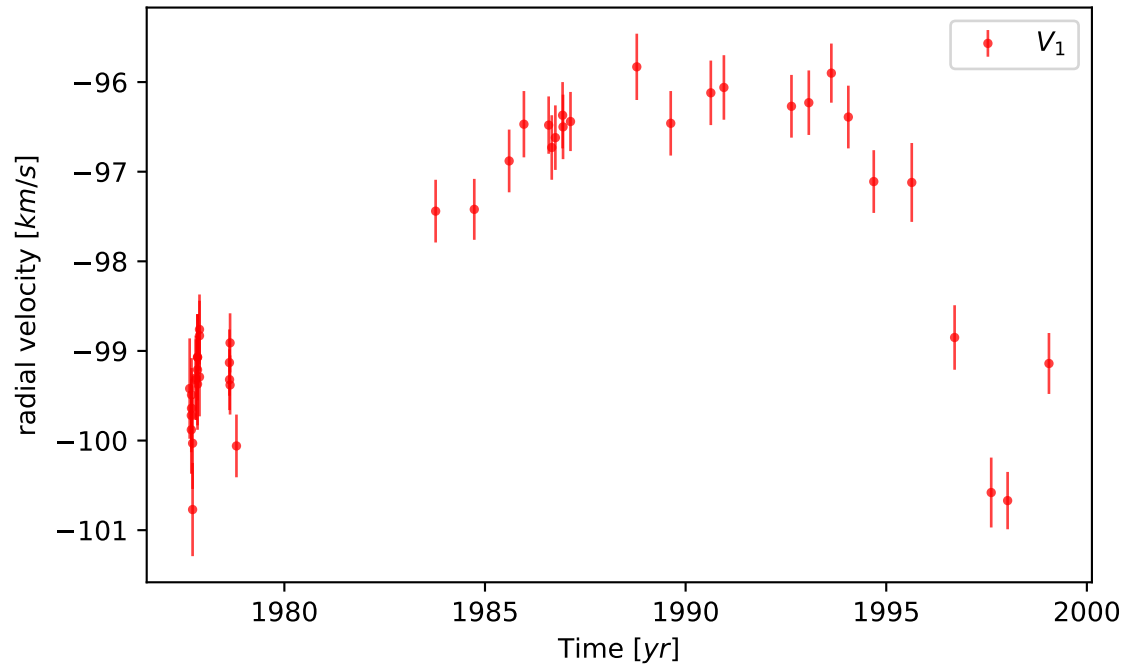
Spectroscopy
