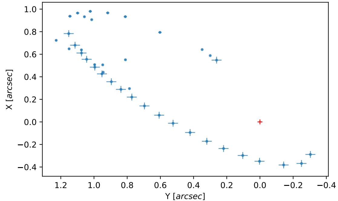
Astrometry
