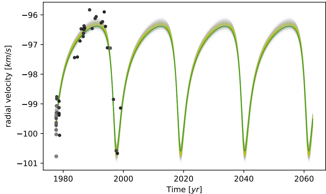
Radial Velocity
