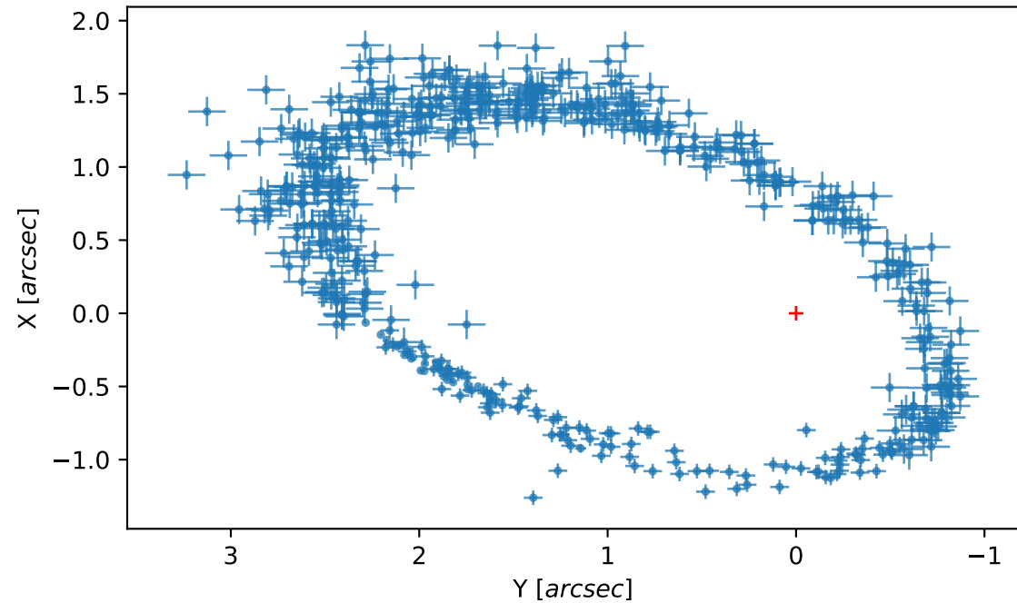
Astrometry
