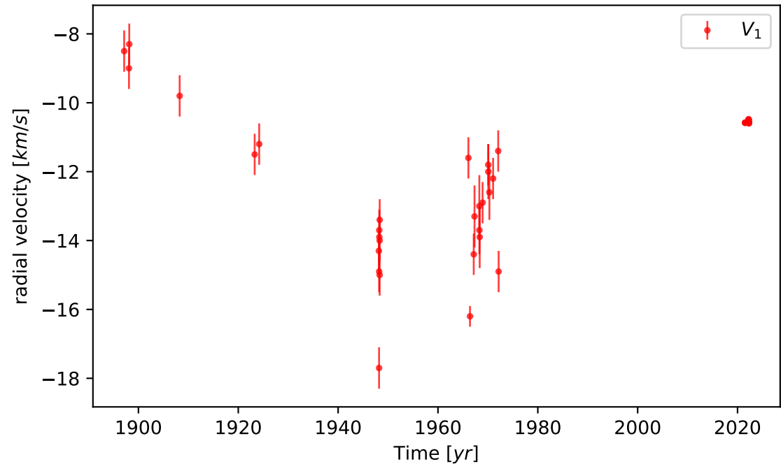
Spectroscopy
