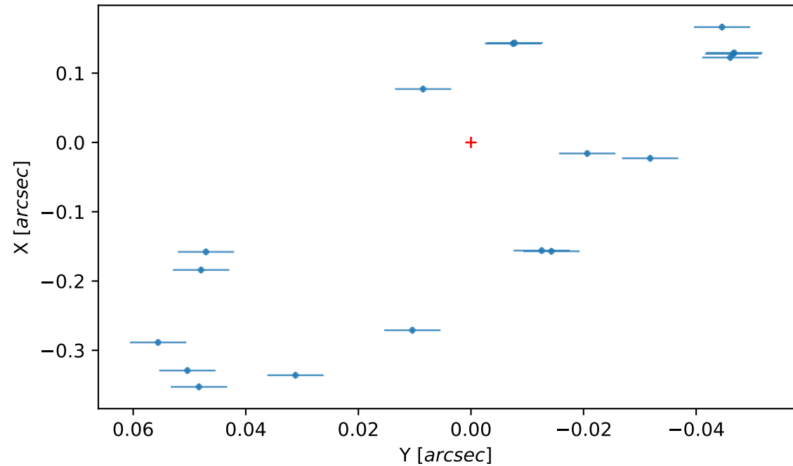
Astrometry
