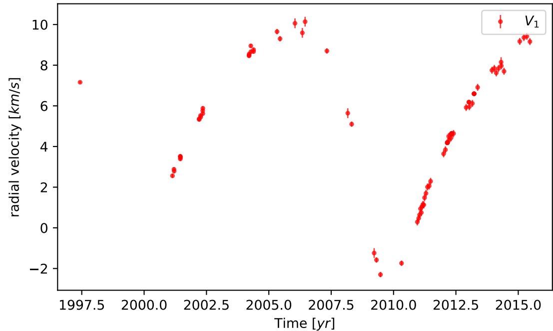
Spectroscopy
