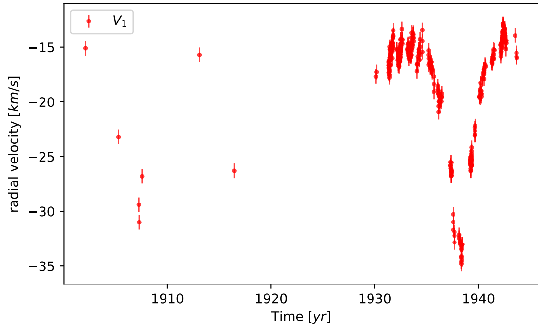
Spectroscopy
