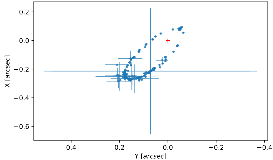
Astrometry
