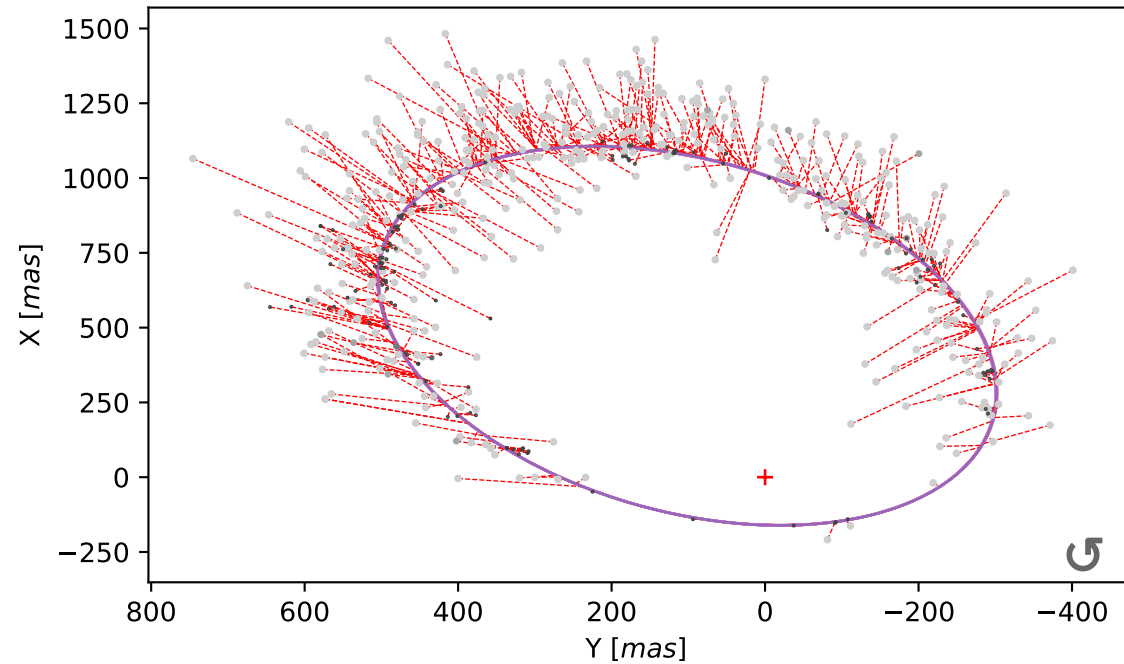
Orbit
