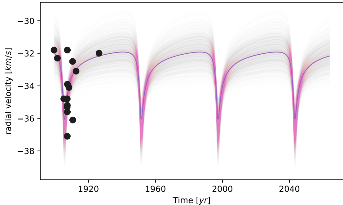
Radial Velocity
