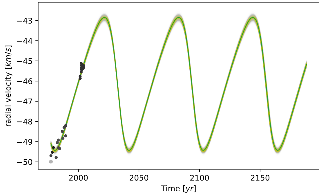
Radial Velocity
