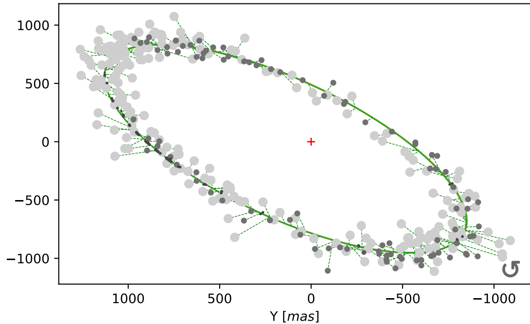
Orbit
