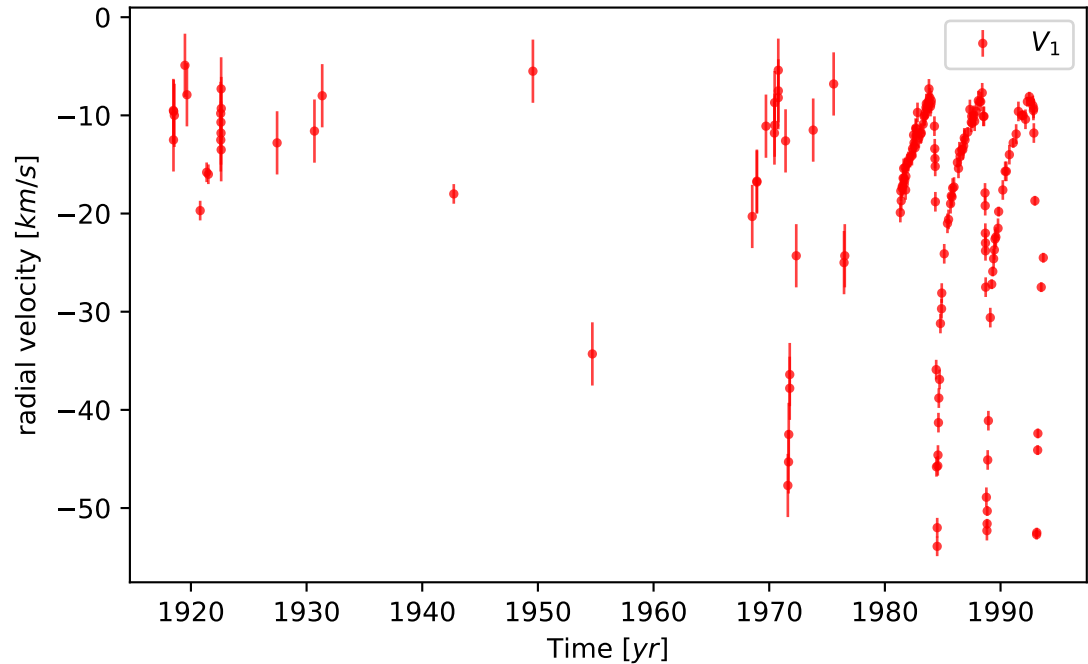
Spectroscopy
