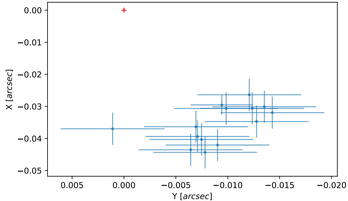
Astrometry
