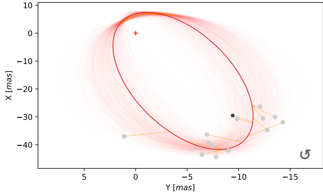
Orbit
