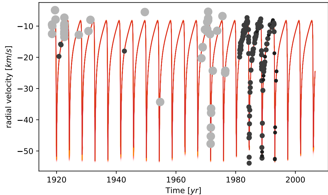
Radial Velocity
