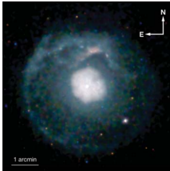
Chandra X-Rays en SNR G21.5-0.9
