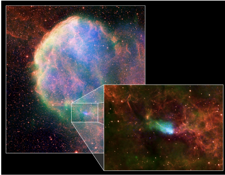
IC 443 SNR - composite Chandra+VLA (Fransson+ 2015, ApJL, 806, L19).
